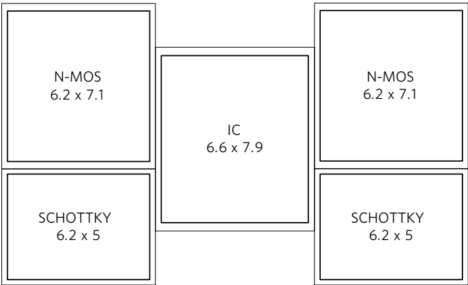
Figure 3. Non-Synchronous Rectification Solution Footprint (264mm 2 )
