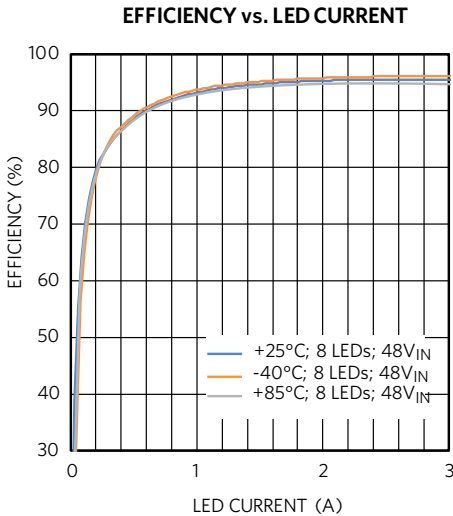
Figure 6. LED Driver Solution Efficiency vs. Load Current
