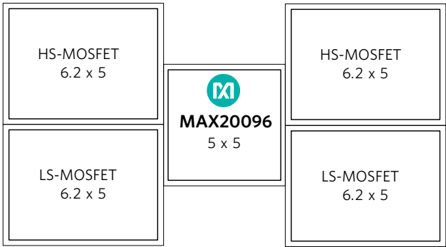
Figure 5. Synchronous Rectification Solution Footprint (149mm 2 )
